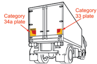
Rigid truck with Category 34A & 33 plates
