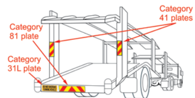
Vehicle carrier with 31L & vertical & horizontal strip plates
