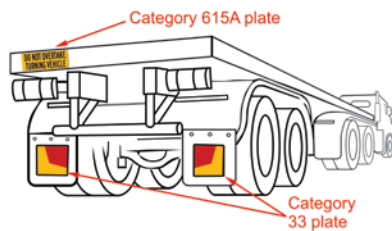
Semitrailer/flat deck vehicle with Category 33 & 31L plates
