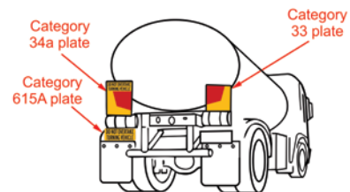
Road tank vehicle with Category 33 plates
